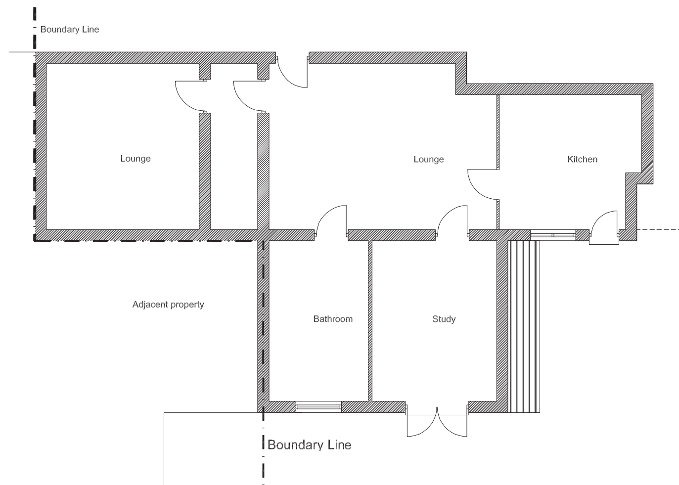
EXISTING GENERAL ARRANGEMENT 1:50 Scale
